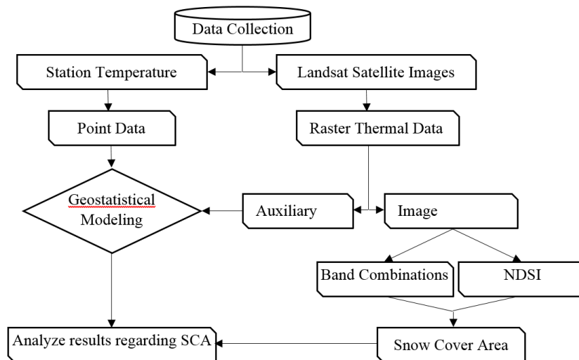
Fig. 2. Methodology Flowchart
