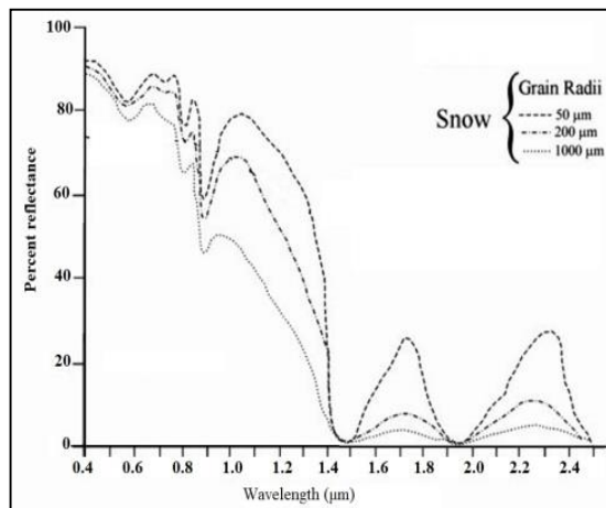
Fig. 4. Snow spectral reflectance. Snow shows variation in spectral reflectance according to the size of crystals in µ (Farooq, 2015).
